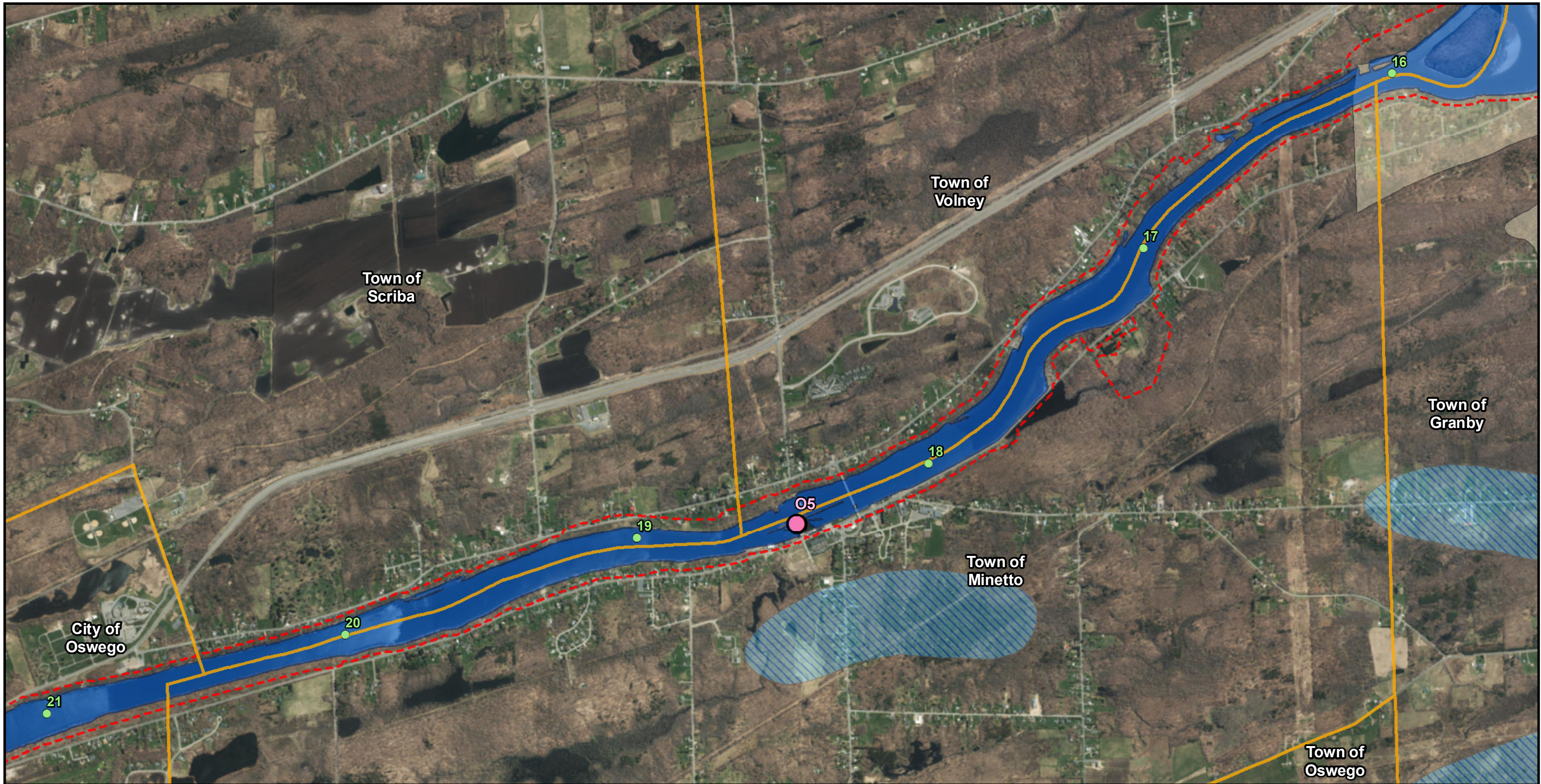
Figure 66F: Aquifers
